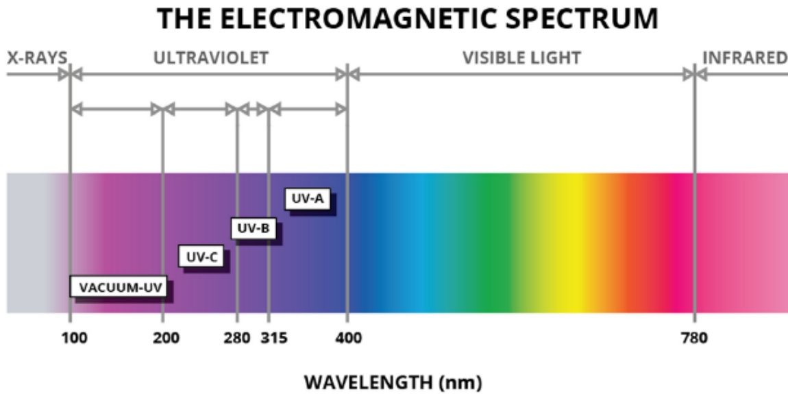
Figure: Displays the different Wavelength of Electromagnetic Spectrum
