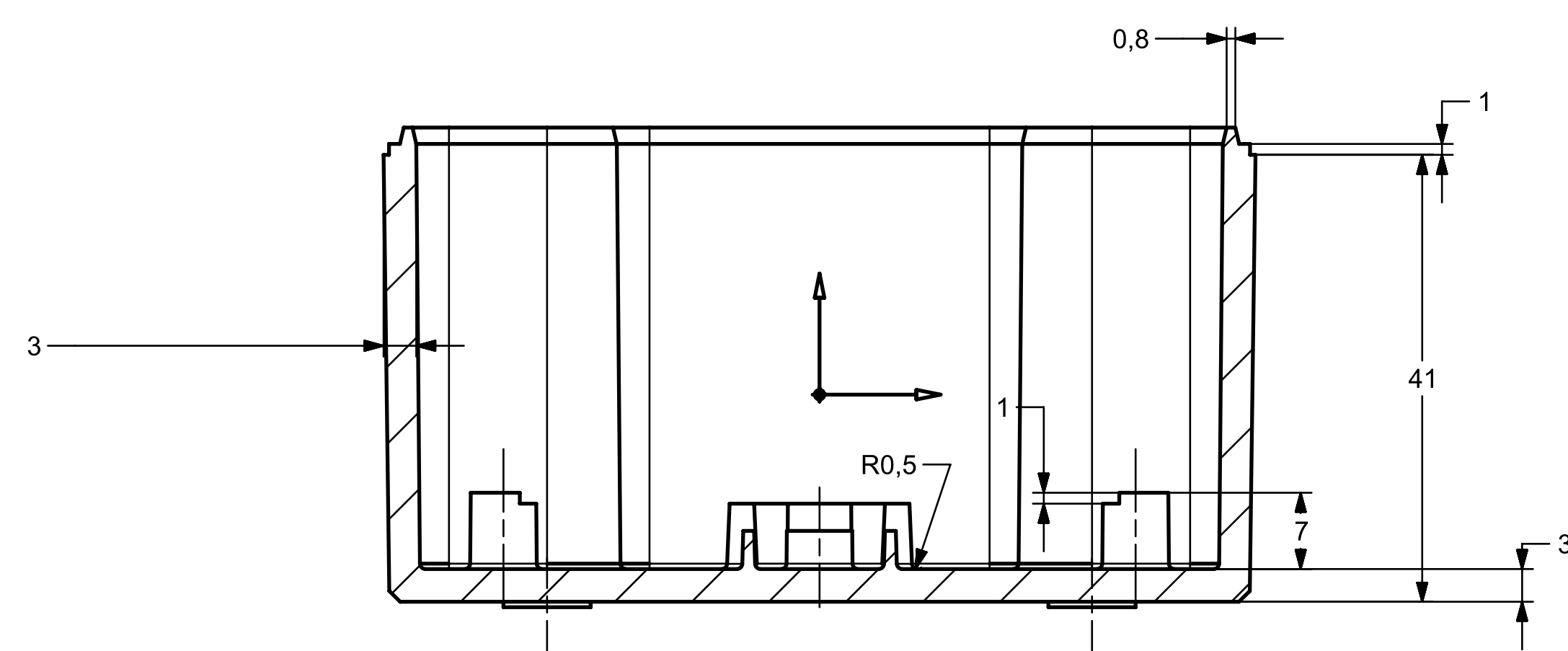
SECTION B-B
