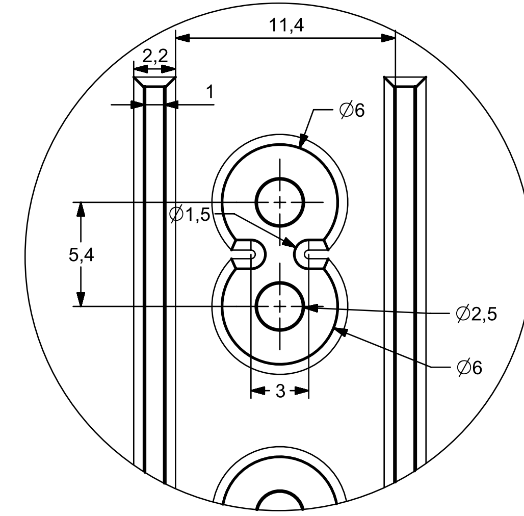
DETAIL E SCALE 5:1
