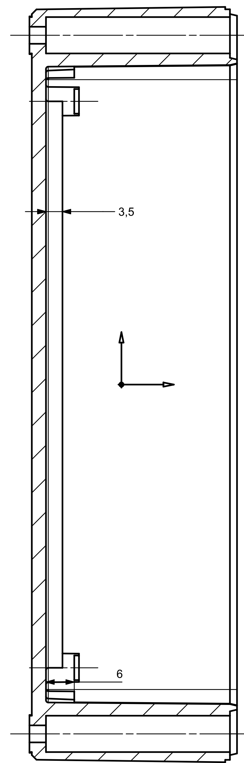
SECTION C-C
