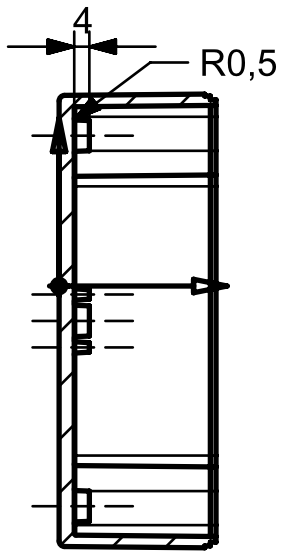
DETAIL C SCALE 1:1
